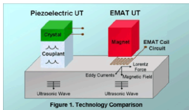
Figure 2. EMAT is couplant-free ultrasonic inspection technique.
